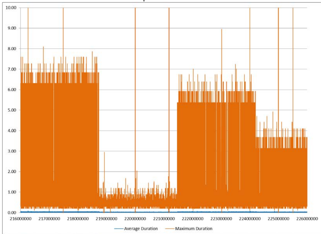
Duration Profile CSX 985 Engine Idle Figure 28
