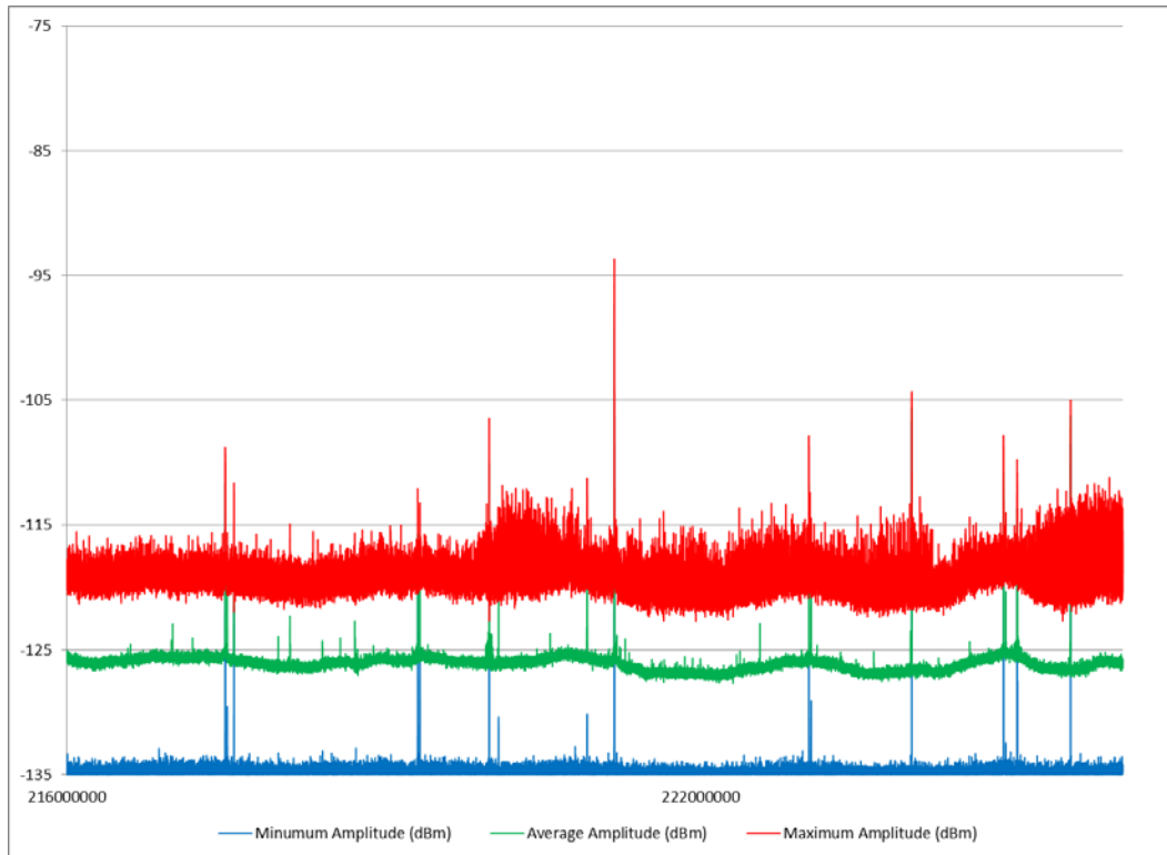
Amplitude Profile
