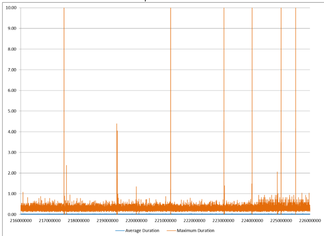
Duration Profile NS 8898 Notch 3 Figure 28
