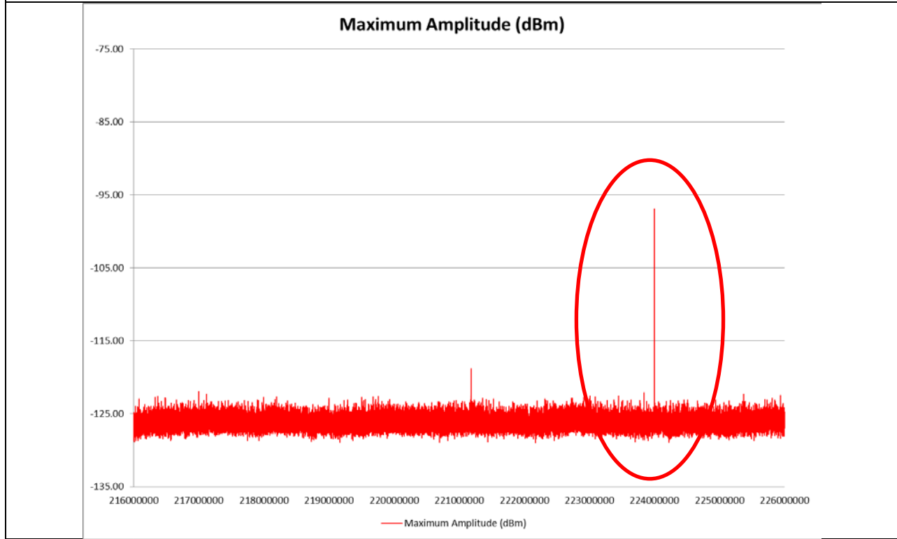
HOT/EOT RX with VHF TX
