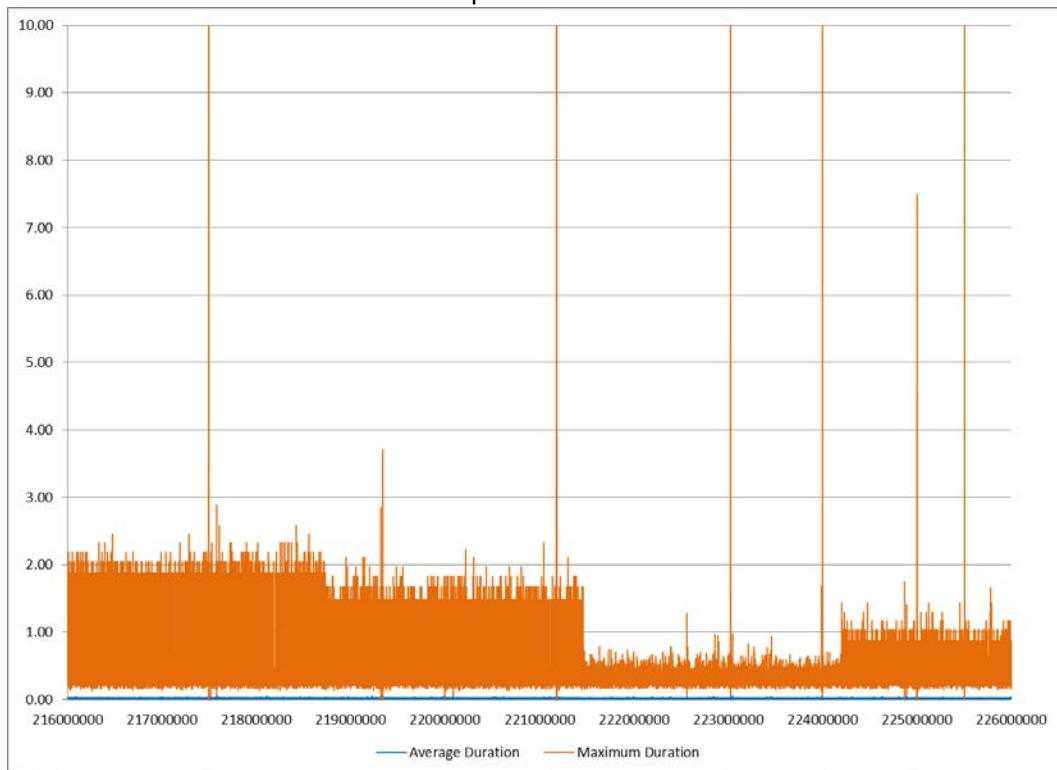
Duration Profile NS 8898 Notch 2 Figure 27
