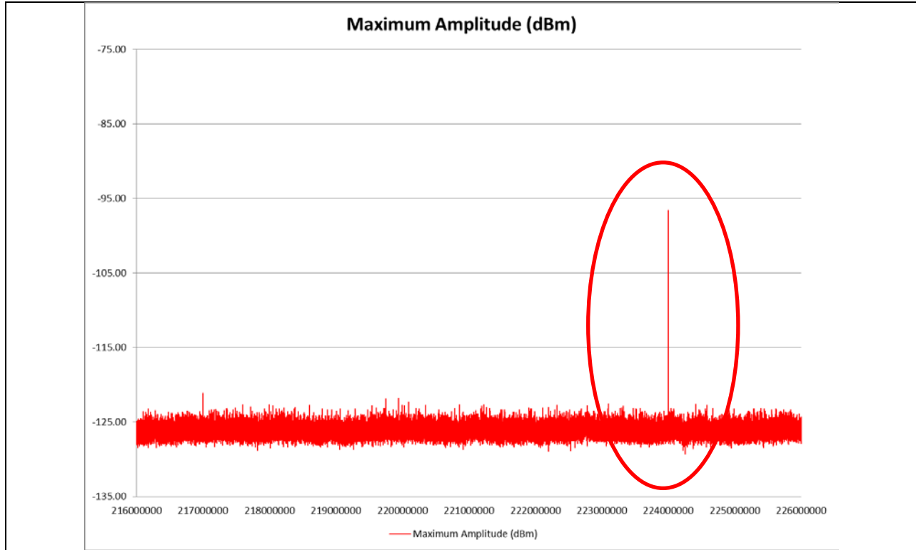
VHF RX with HOT/EOT TX
