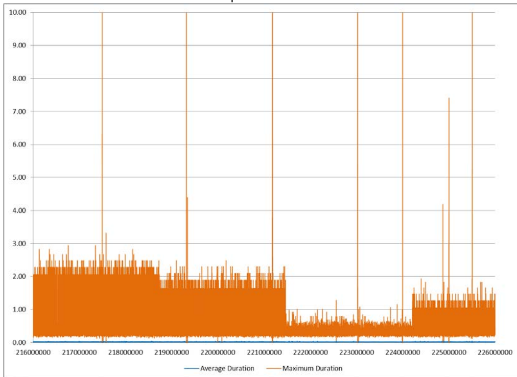
Duration Profile NS 8898 Notch 6 Figure 31
