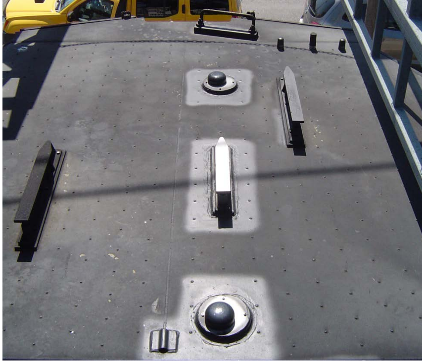
NS 8898 Rooftop View Front Facing
