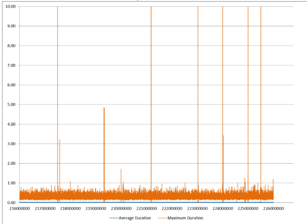
Duration Profile NS 8898 Notch 1 Figure 26
