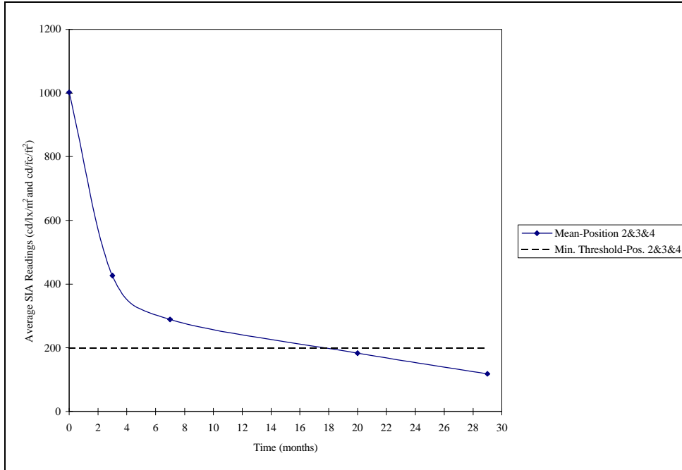
Figure 5-9. NS Double Stack Cars – Mean Degradation Trend for Positions 2, 3, and 4
