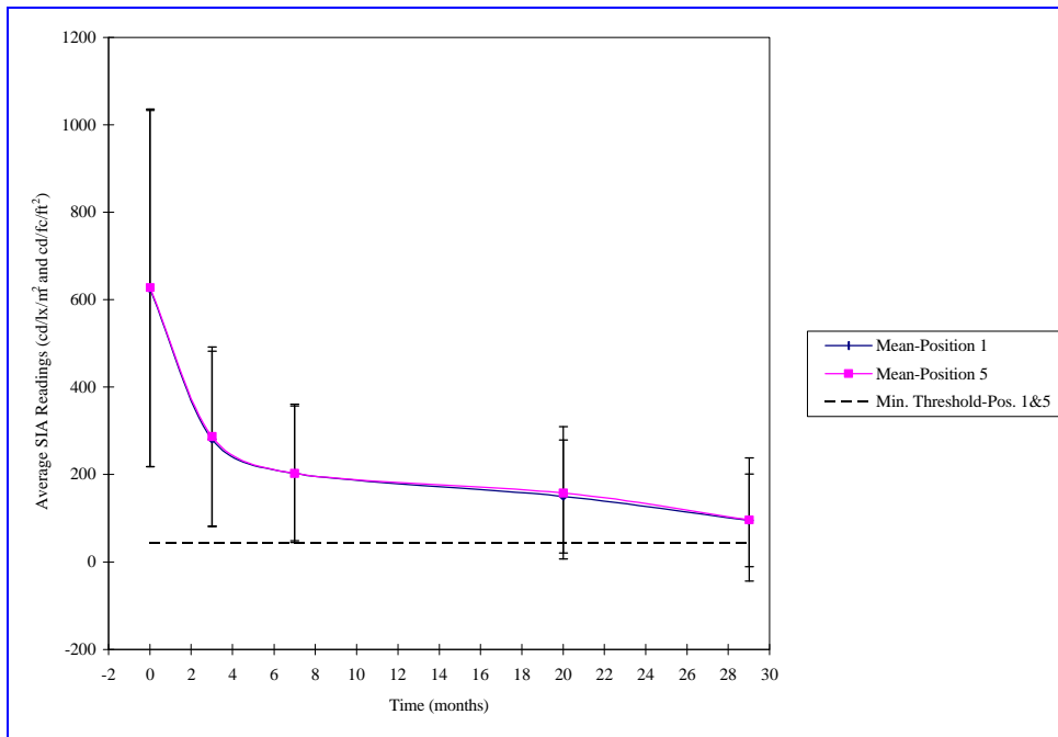
Figure 5-8. NS Double Stack Cars – Degradation of Positions 1 and 5
