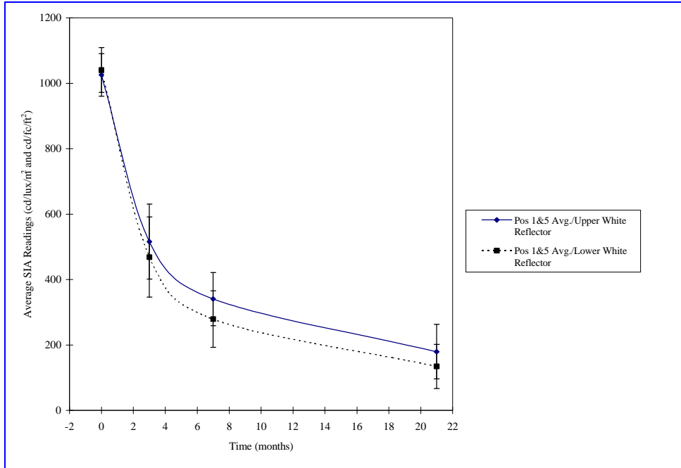
Figure 5-25. Hopper Car – Upper and Lower White Reflector Degradation Rates
