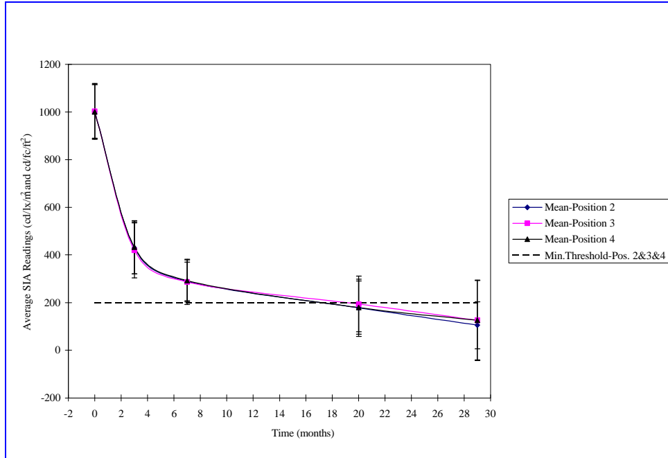
Figure 5-7. NS Double Stack Cars – Degradation of Positions 2, 3, and 4
