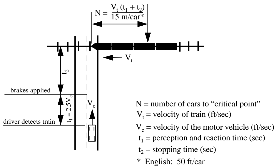
Figure 3-1. Relationship between “Critical Point” on Train and Perception/Reaction and Stopping
