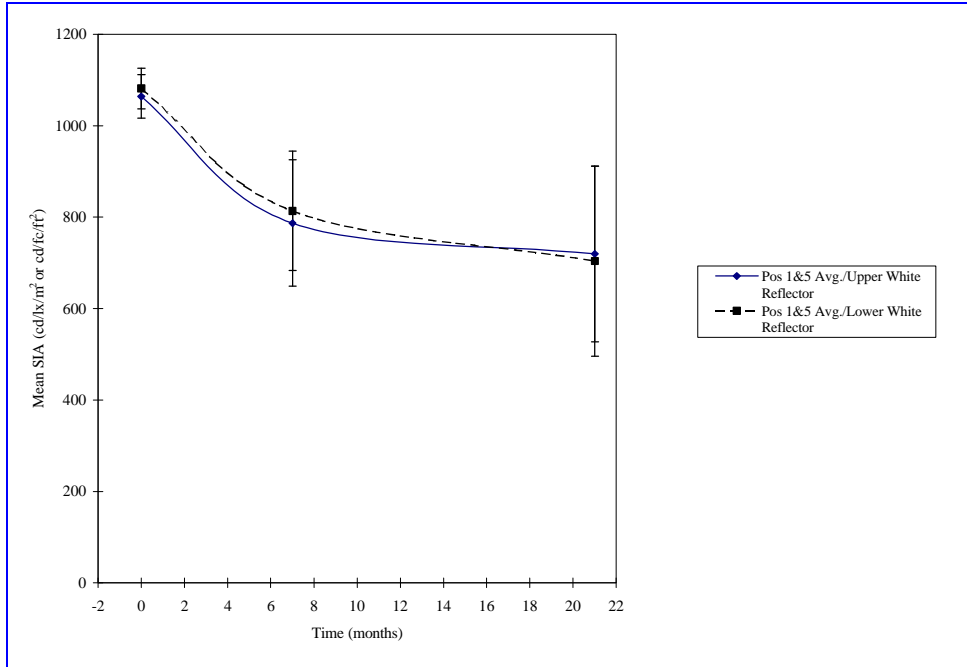
Figure 5-23. Tank Car – Upper and Lower White Reflector Degradation Rates
