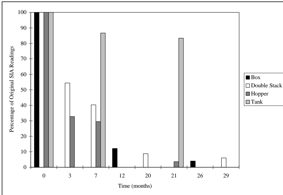
Figure 5-19. Comparative Degradation Rates for All Freight Car Types in Positions 1 and 5
