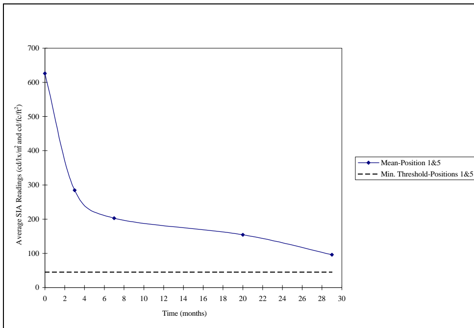
Figure 5-10. NS Double Stack Cars – Mean Degradation Trend for Positions 1 and 5
