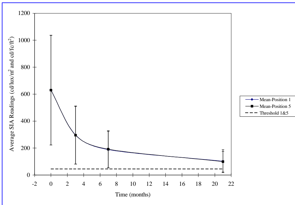
Figure 5-12. NS Hopper Cars – Degradation of Positions 1 and 5
