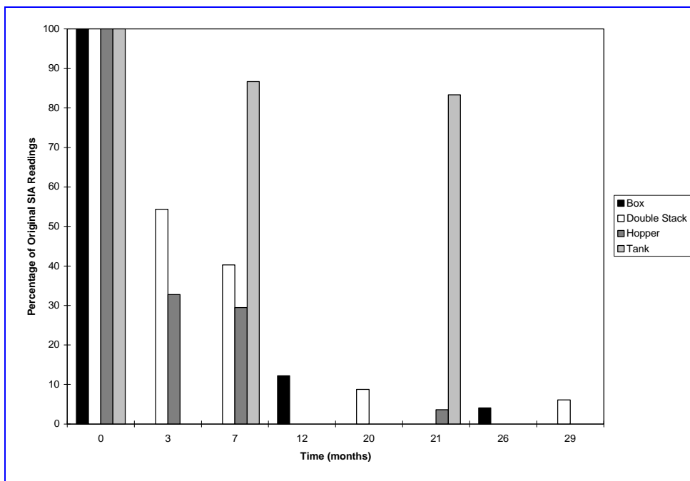
Figure 5-20. Comparative Degradation Rates for All Freight Car Types in Position 2
