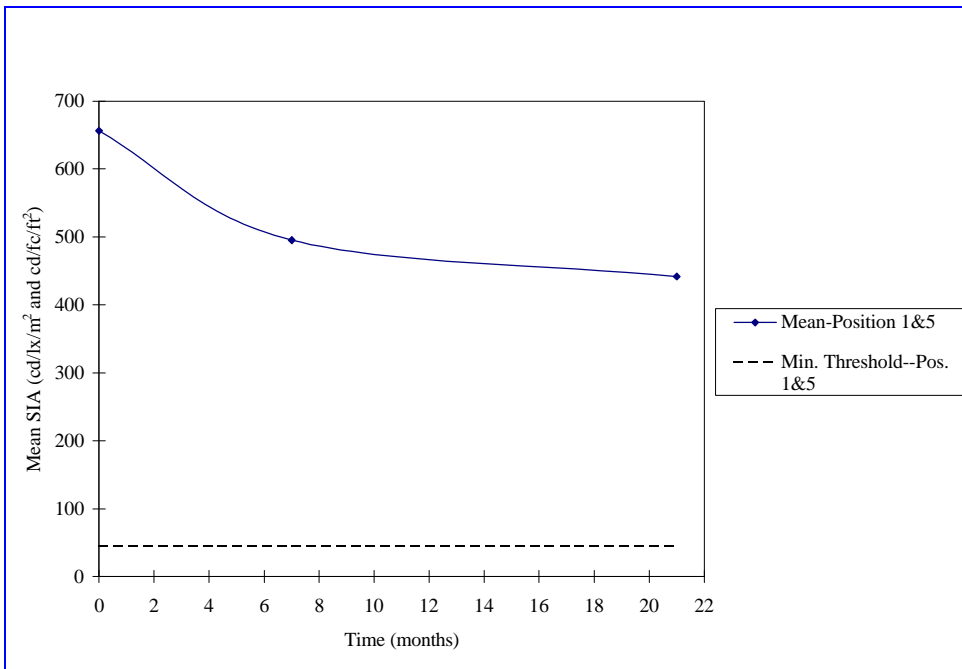
Figure 5-4. Alaska Tank Cars – Mean Degradation Trend for Positions 1 and 5
