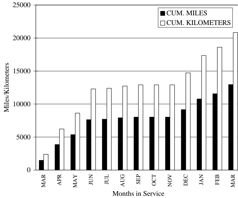
Figure 4-17. Cumulative Mileage
