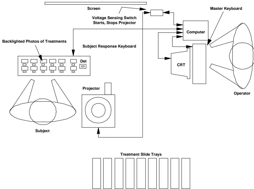
Figure 6-4. Layout of Experiment
