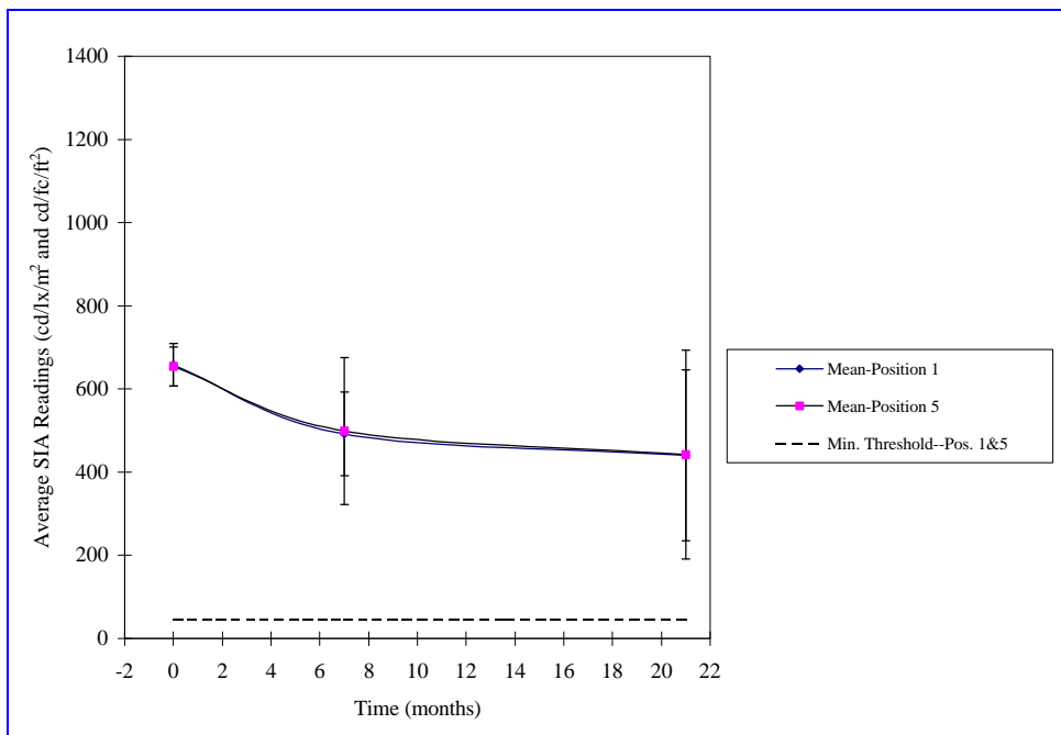
Figure 5-2. Alaska Tank Cars – Degradation of Positions 1 and 5
