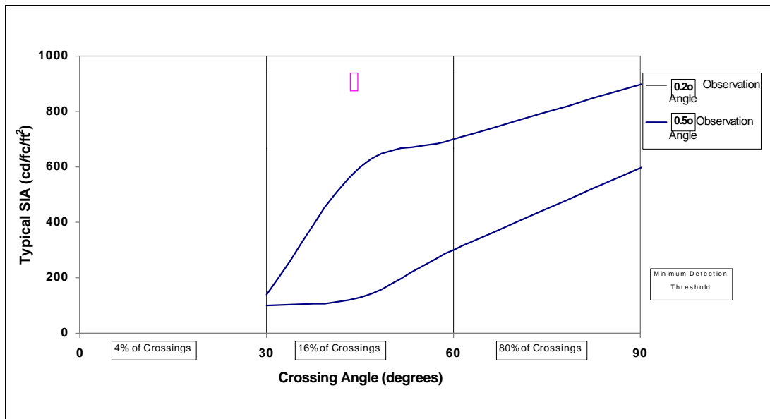
Figure 6. Typical Coefficients of Retroreflection for 3M's 981 sheeting series as a function of grade crossing angle (white 4" x 8")
