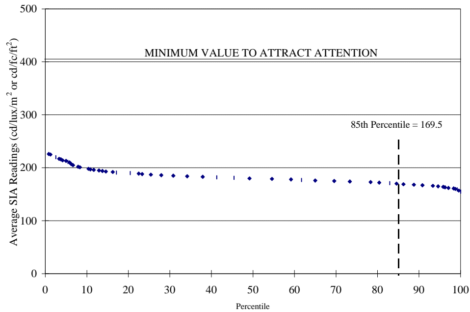
Figure 4-13. Unwashed Red Prismatic (Mean and One Standard Deviation and Percentiles)
