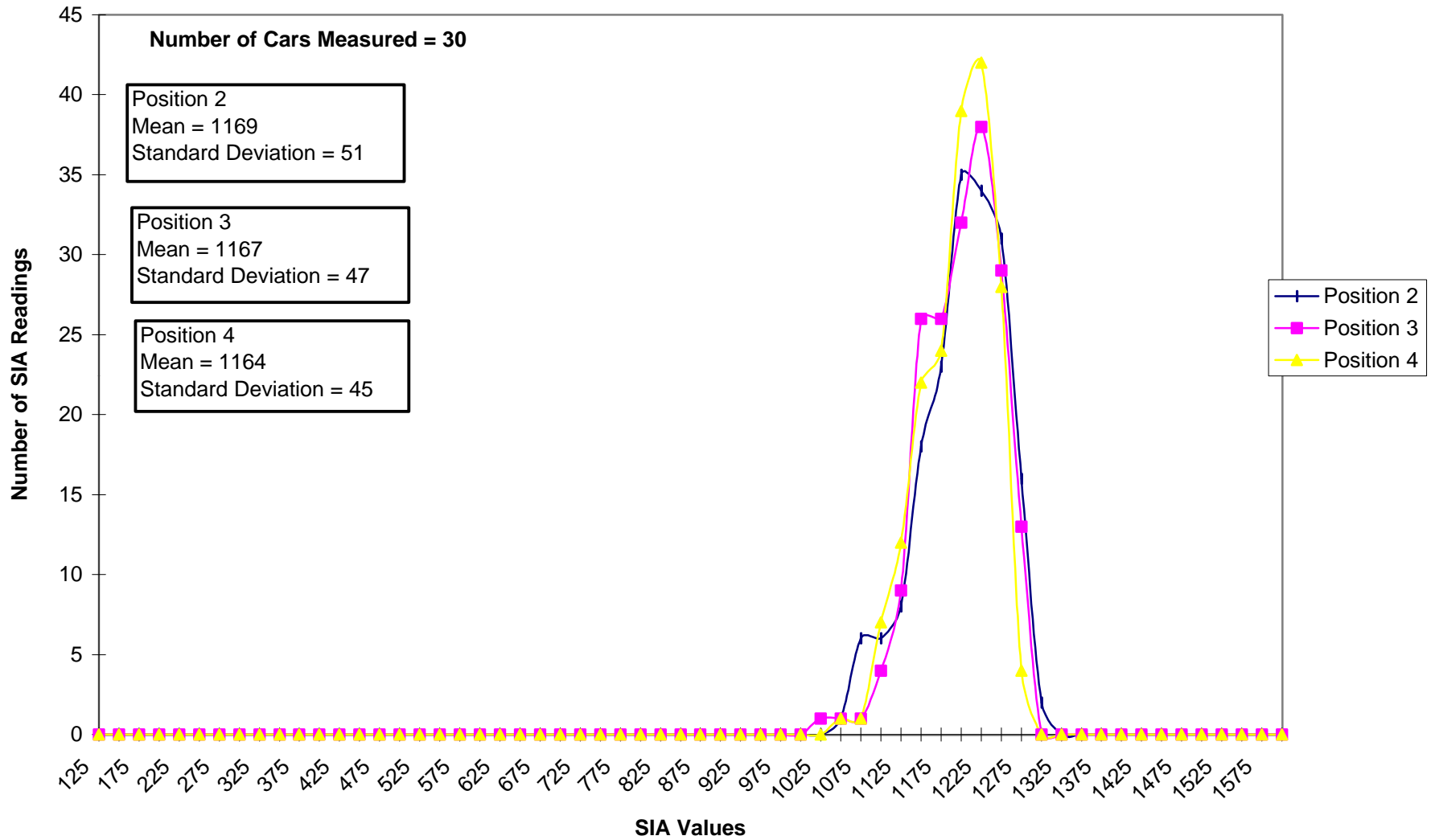
Tank Car Data - Month '0': Number of SIA Readings vs. Average SIA Values for Positions 2, 3, &4
