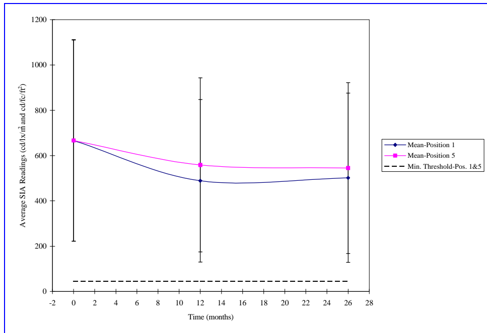
Figure 5-16. NS Box Cars – Degradation of Positions 1 and 5
