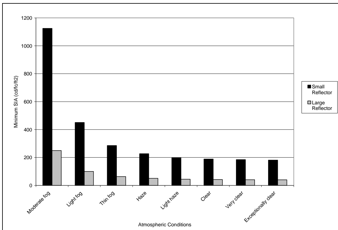
Figure 2. Effects of atmospheric conditions on minimum detection levels for both the small (4" x 8") and the large (4" x 36") reflectors.
