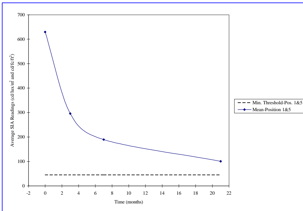
Figure 5-14. NS Hopper Cars – Mean Degradation Trend for Positions 1 and 5
