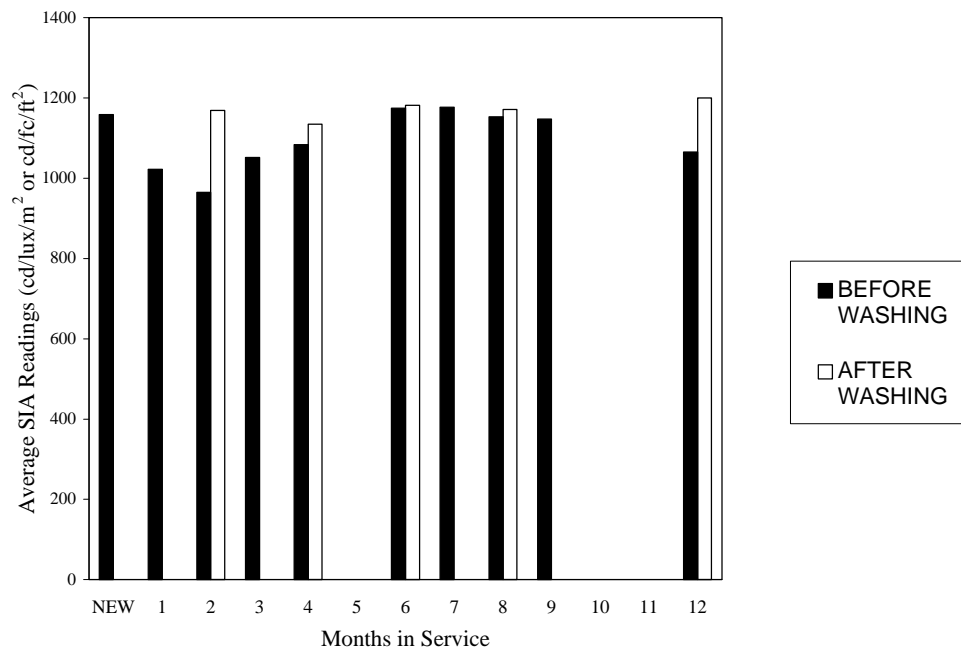
Figure 4-15. SIA of Prismatic Decals with One- and Two-Month Washing Cycles
