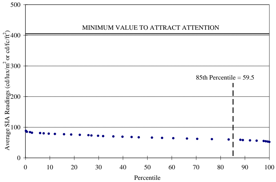
Figure 4-12. Unwashed Prismatic vs. Unwashed Enclosed Lens (Percentiles)
