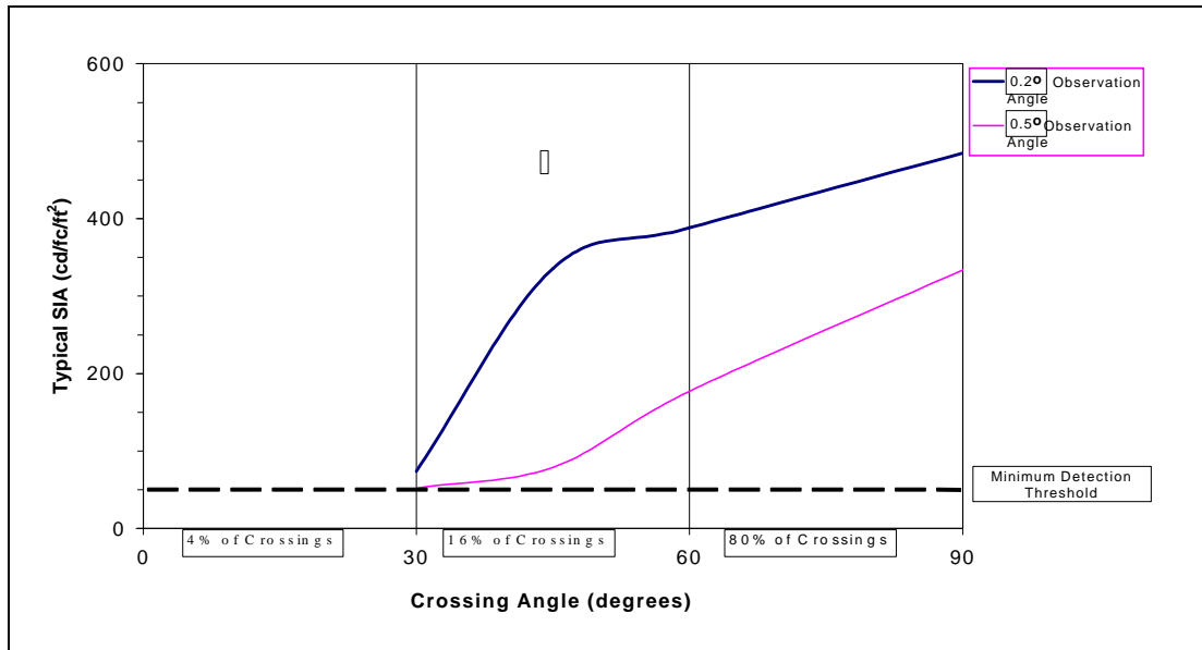
Figure 7. Typical Coefficients of Retroreflection for 3M's 981 sheeting series as a function of grade crossing angle (red & white 4" x 36")
