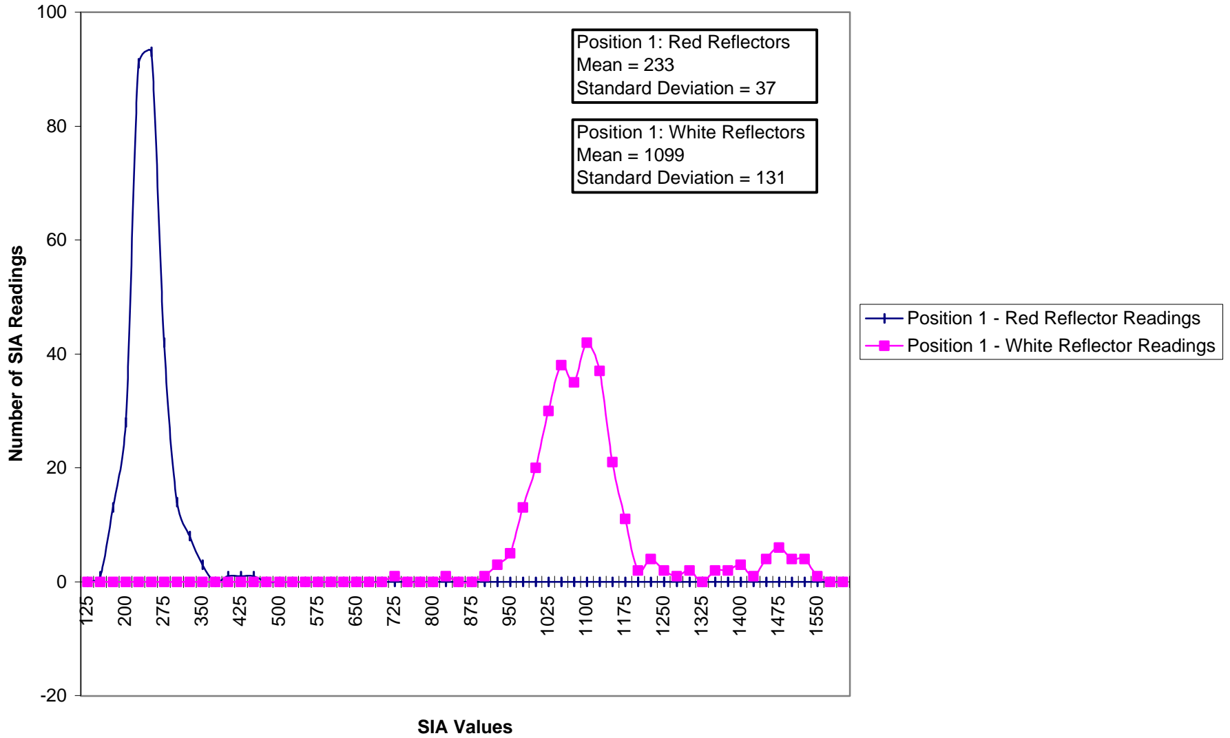
Box Car Data - Month '0': Number of SIA Readings vs. SIA Values of Red and White Reflectors for Position 1
