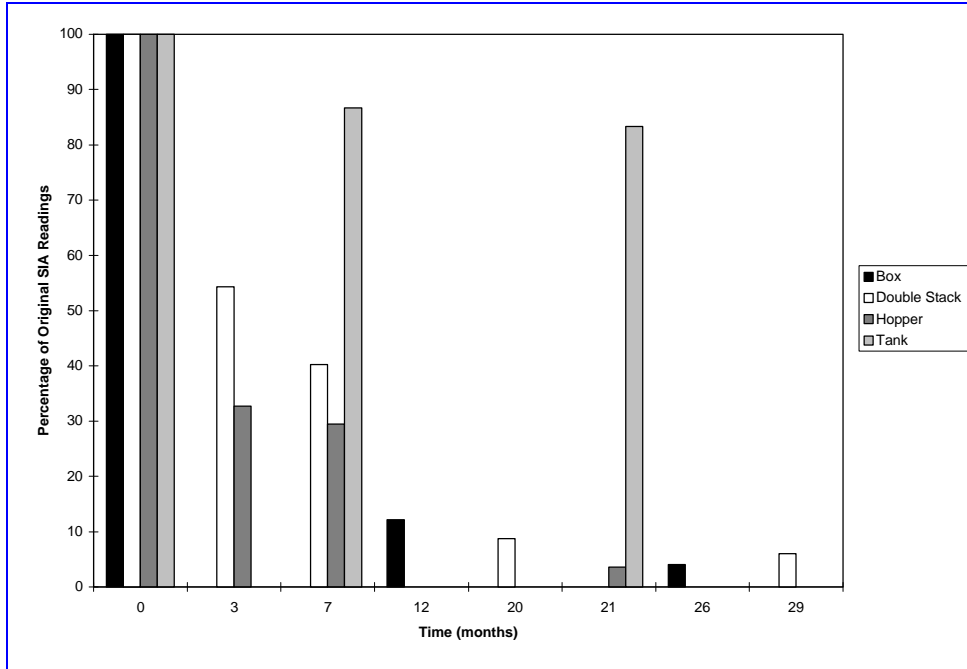
Figure 5-21. Comparative Degradation Rates for All Freight Car Types in Position 3
