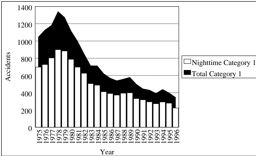
Figure 1-4. Trend in Nighttime Category 1 RIT Accidents versus Total Category 1 RIT Accidents (1975–1996)
