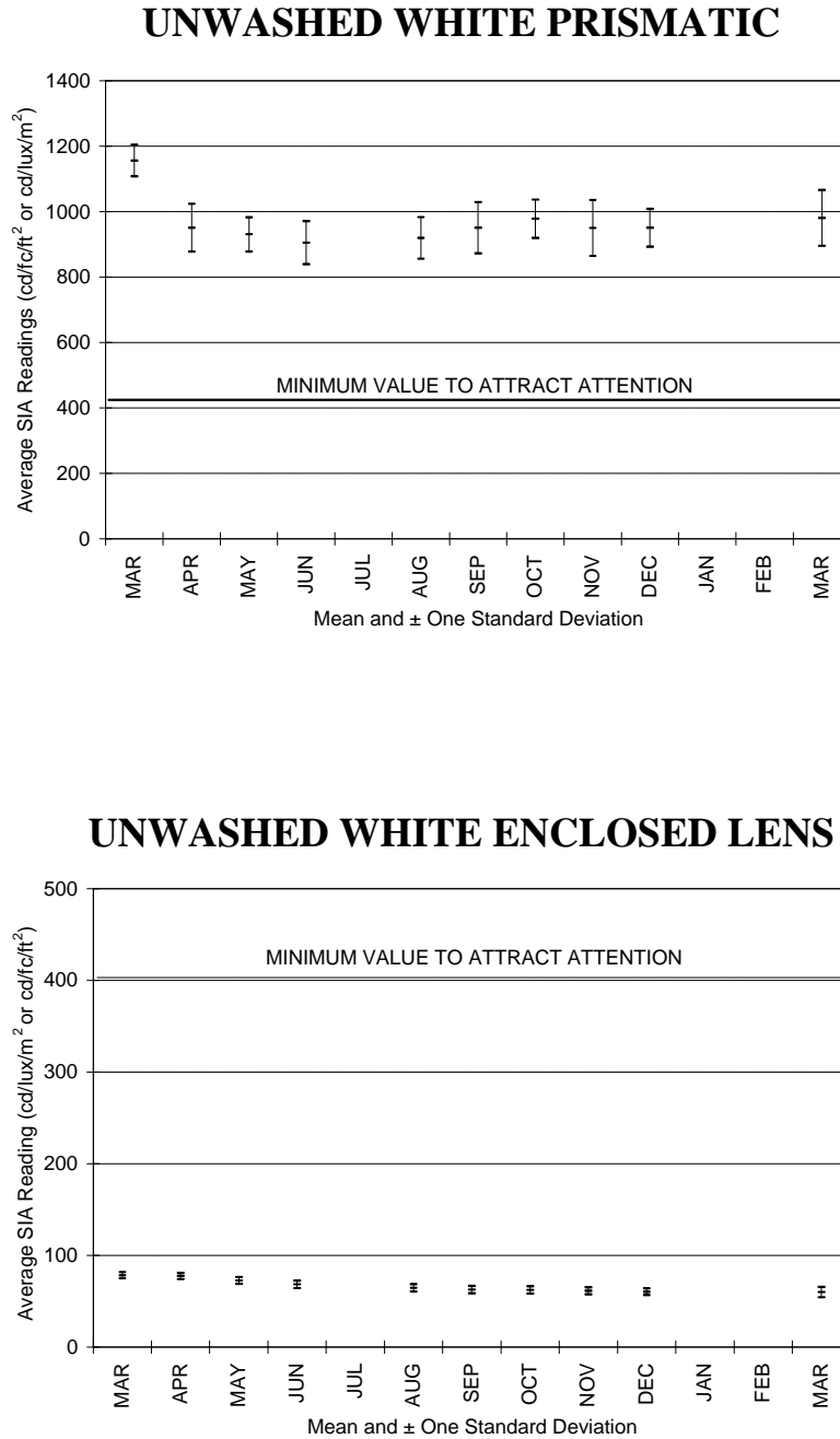
Figure 4-11. Unwashed Prismatic vs. Unwashed Enclosed Lens (Mean and One Standard Deviation)
