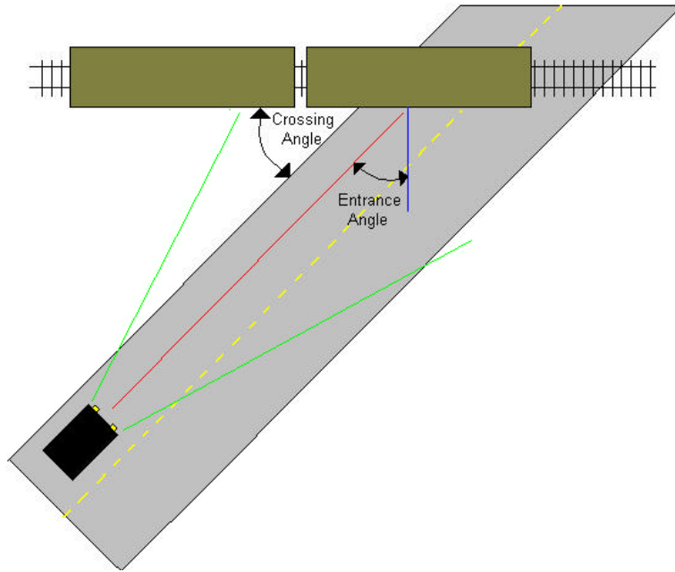
Figure 5. Top view of highway/rail intersection without roadway curvature (tangent).
