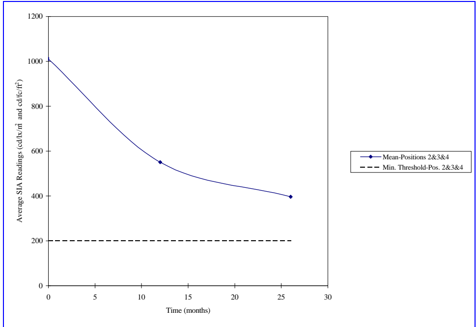
Figure 5-17. NS Box Cars – Mean Degradation Trend for Positions 2, 3, and 4
