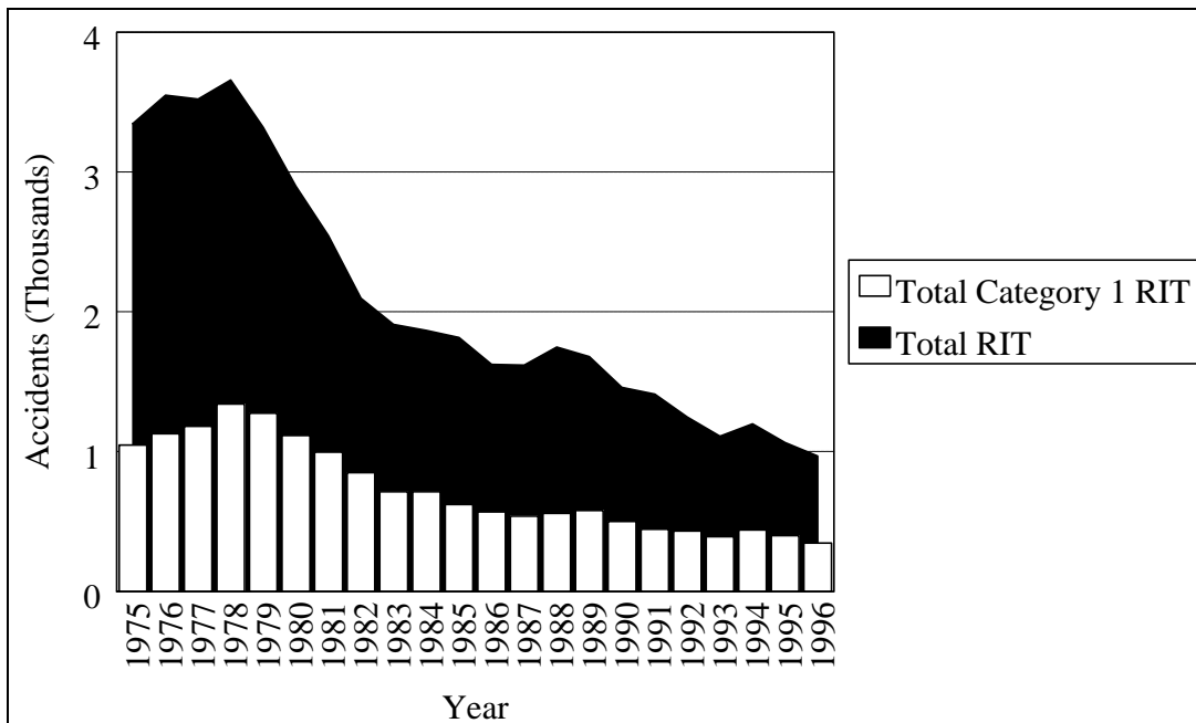
Figure 1-3. Trend in Total Category 1 Accidents versus Total RIT Accidents (1975–1996)
