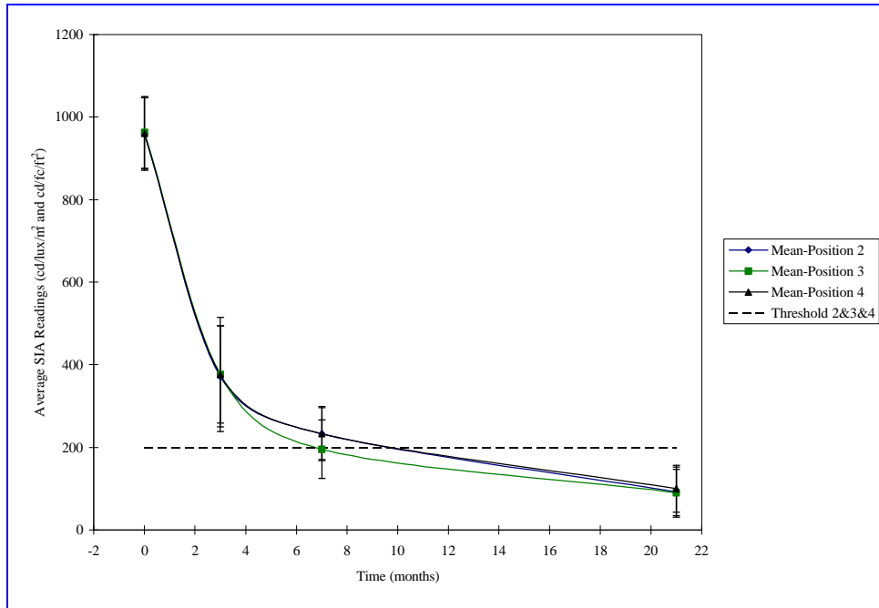
Figure 5-11. NS Hopper Cars – Degradation of Positions 2, 3, and 4
