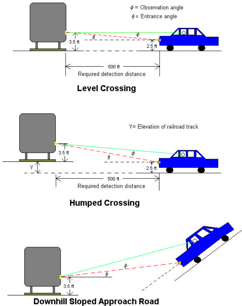
Figure 3. Side view of various highway-rail crossing geometry
