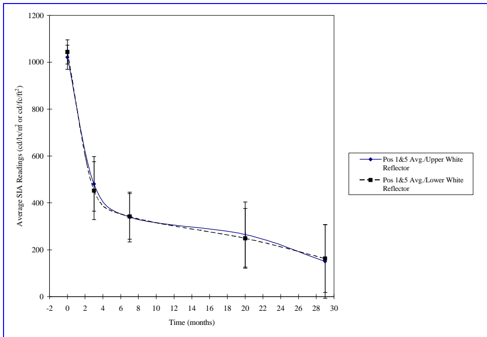
Figure 5-24. Double Stack Car – Upper and Lower White Reflector Degradation Rates
