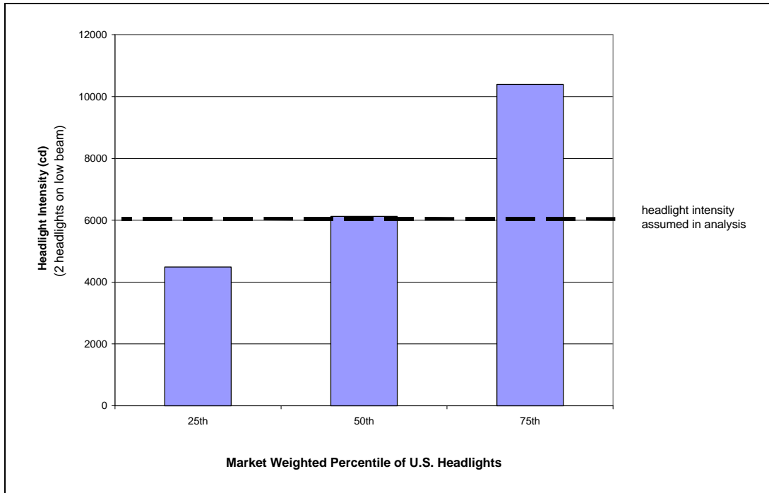
Figure 1. Light intensities from pairs of low beam headlights at freight car reflector location, from a market-weighted database of U.S. headlights (Savik, 1997)
