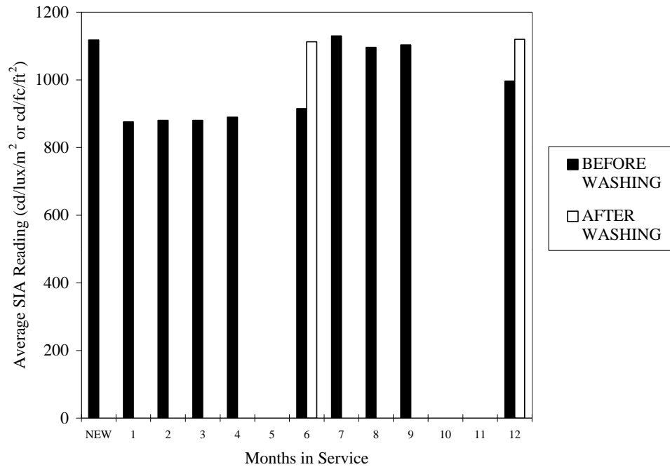
Figure 4-16. SIA of Decals with Four- and Six-Month Washing Cycles
