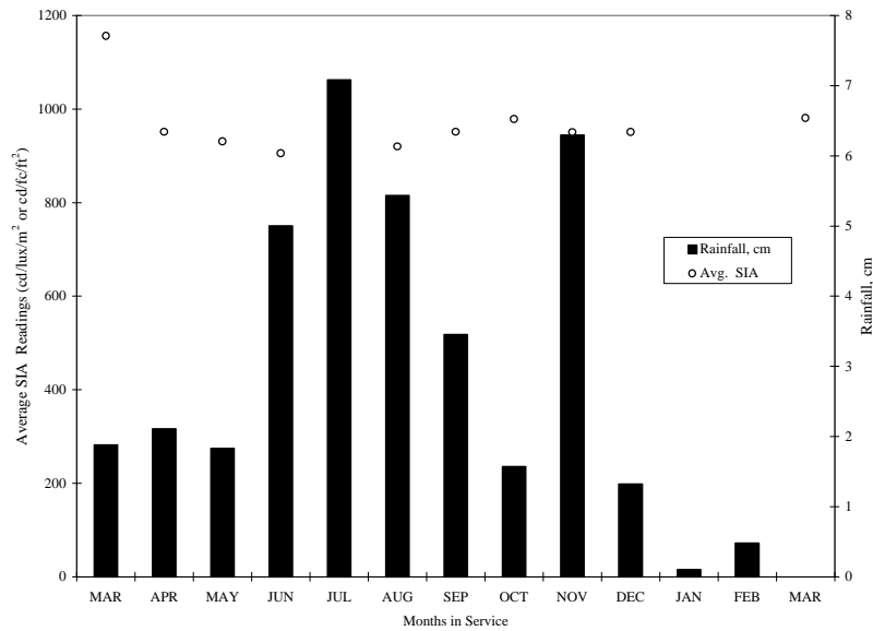
Figure 4-19. SIA vs. Rainfall and Snowfall 1
