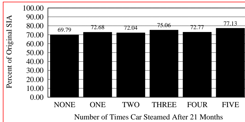
Figure 5-6. Effects on Tank Car Reflectors from Internal Steam Cleaning
