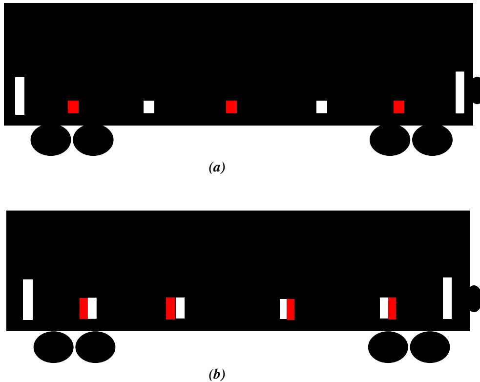
Figure 7-1. Suggested Improved Reflector Patterns on a Typical Freight Car
