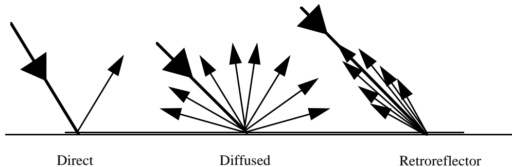
Figure 2-1. Types of Reflectors
