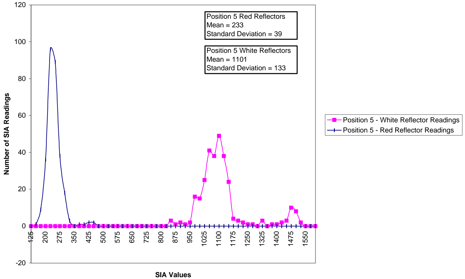
Box Car Data - Month '0': Number of SIA Readings vs. SIA Values of Red and White Reflectors for Position 5
