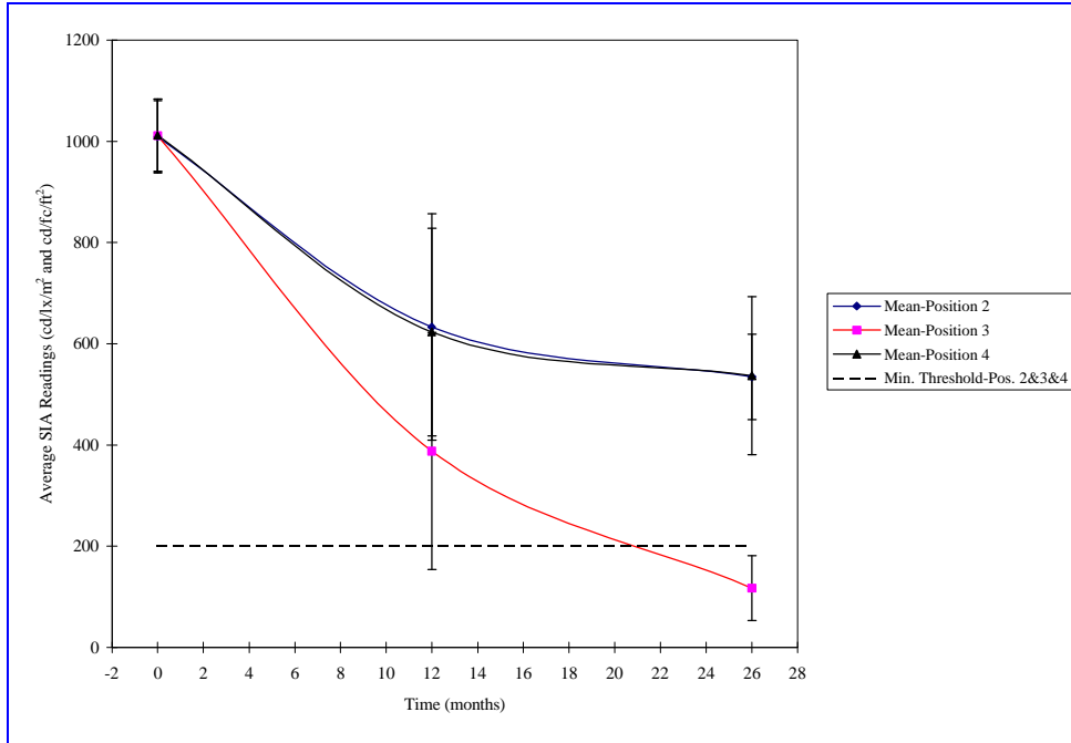
Figure 5-15. NS Box Cars – Degradation of Positions 2, 3, and 4
