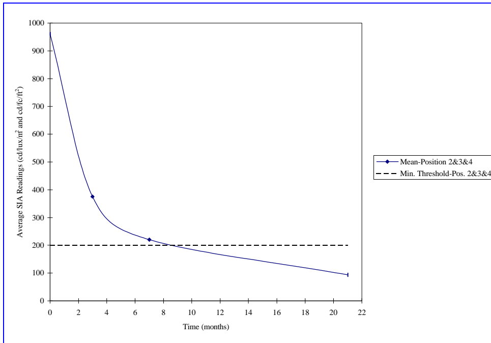
Figure 5-13. NS Hopper Cars – Mean Degradation Trend for Positions 2, 3, and 4
