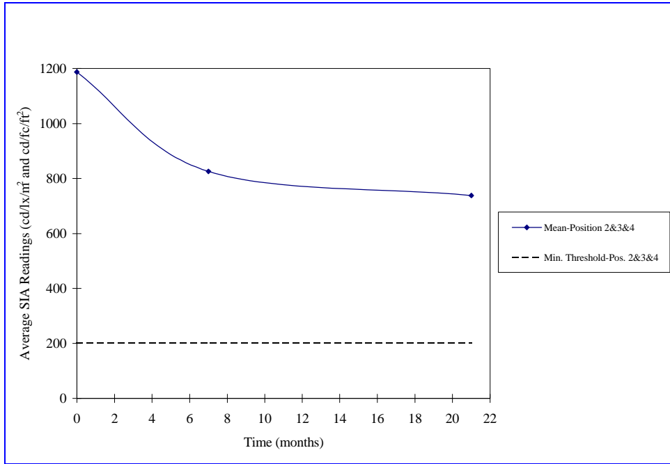
Figure 5-3. Alaska Tank Cars – Mean Degradation Trend for Positions 2, 3, and 4
