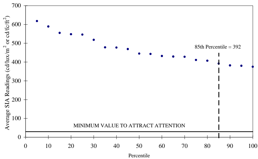
Figure 4-14. Unwashed Red-and-White Prismatic Delineating Stripe (Monthly Averages and Percentiles)
