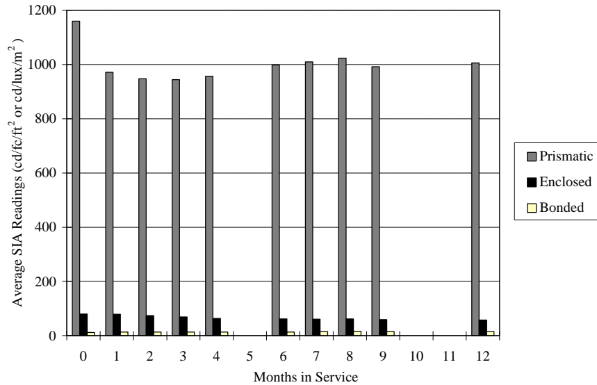
Figure 4-10. Comparison of All Reflective Materials Tested (Unwashed Reference)
