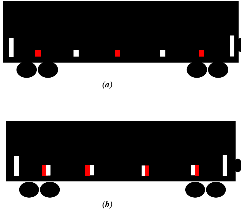
Figure ES-1. Suggested Improved Reflector Patterns on a Typical Freight Car
