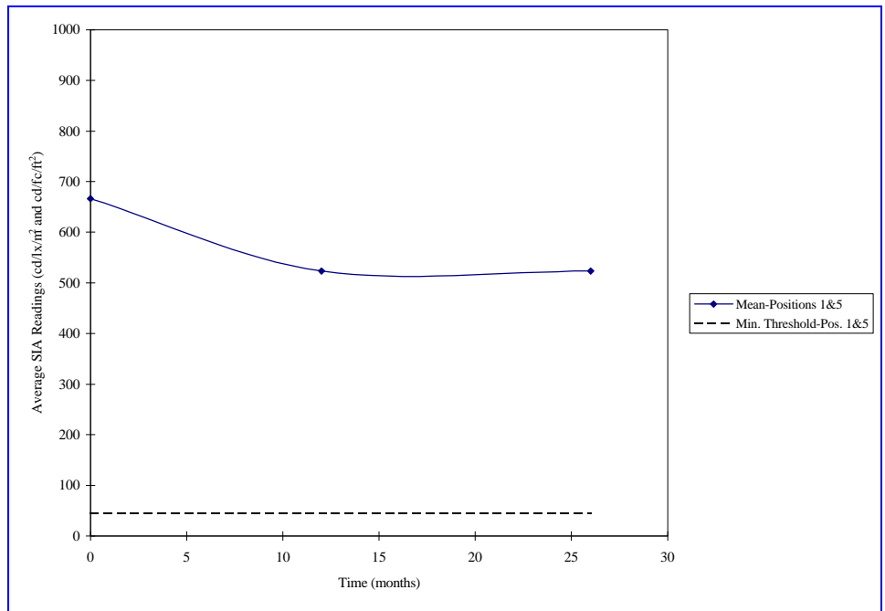
Figure 5-18. NS Box Cars – Mean Degradation Trend for Positions 1 and 5
