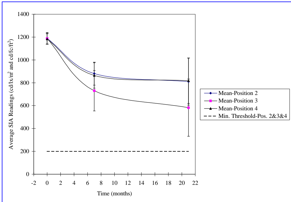
Figure 5-1. Alaska Tank Cars – Degradation of Positions 2, 3, and 4
