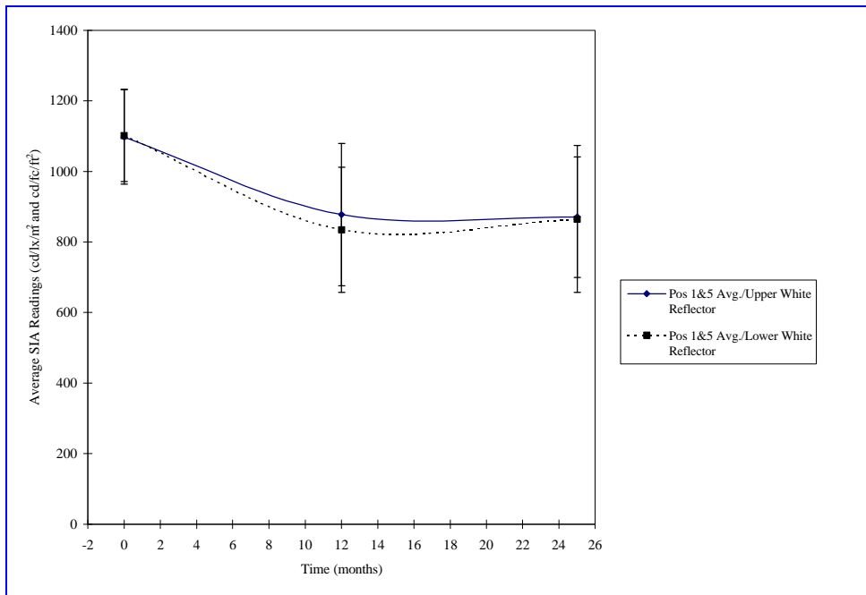
Figure 5-26. Box Car – Upper and Lower White Reflector Degradation Rates
