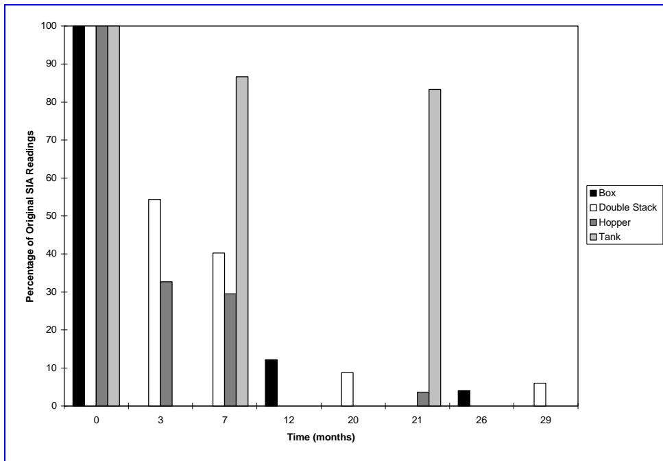
Figure 5-22. Comparative Degradation Rates for All Freight Car Types in Position 4
