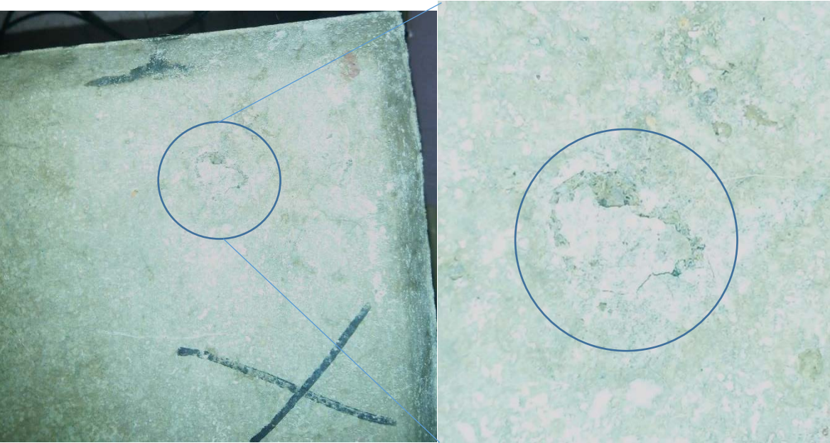
Figure 26: Small pop-out/crack in tie #1-4397-F.
