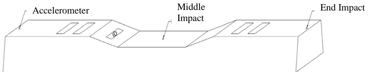
Figure 13: Impact and accelerometer locations on tie top surface.
