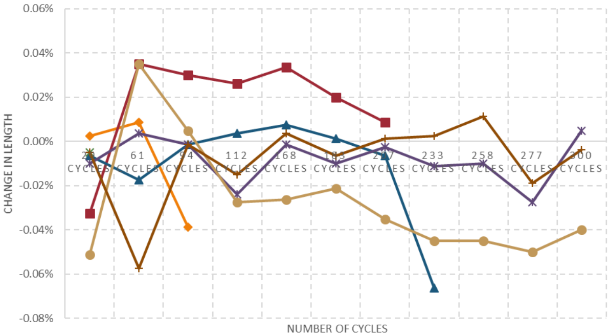
Figure A-3: Length change in horizontal direction at the ID side.
