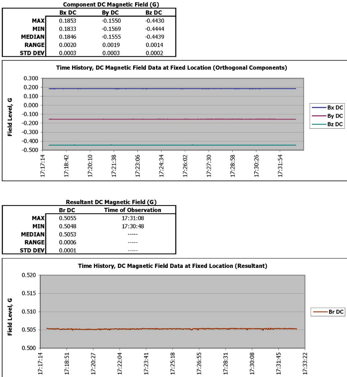
Figure 3.5-A-6(d) Location 04: Static (DC) magnetic field data with temporal statistics
