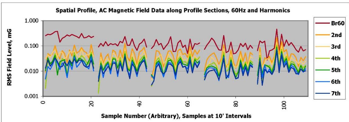
Figure 3.5-A-3(e) Location 01: Low-frequency (AC) magnetic field data with temporal and spatial statistics
