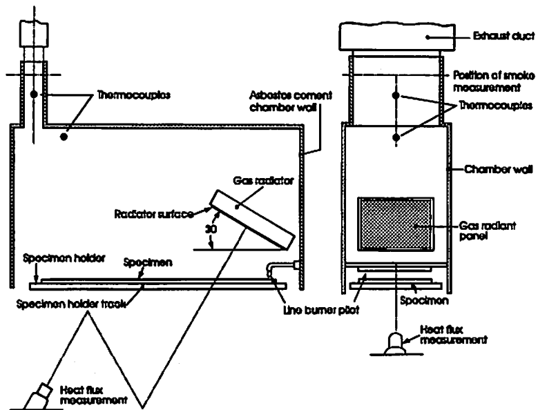
Figure B3. The ASTM E 648 Flooring Radiant Panel Test
