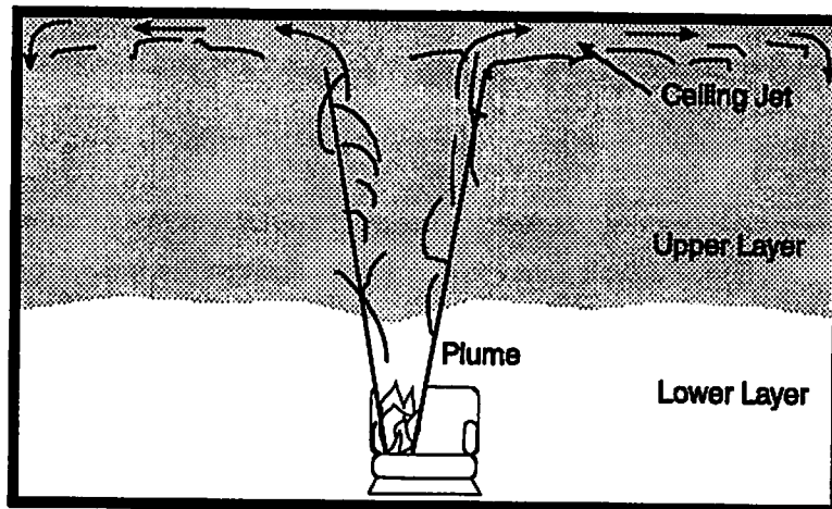
Figure 2. Zone Model Terms.
