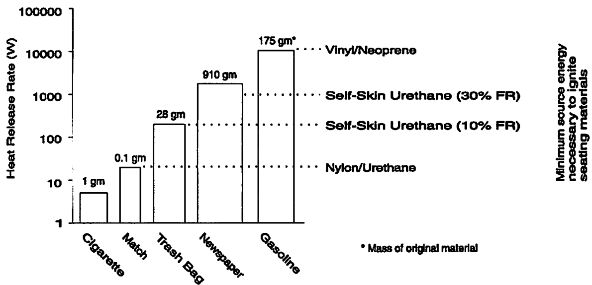
Figure 3. Minimum Ignition Source Energies for Various Seat Assemblies.
