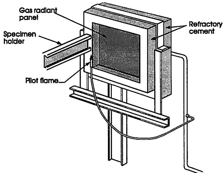
Figure C5. The NF P 92506 Floor Covering Test
