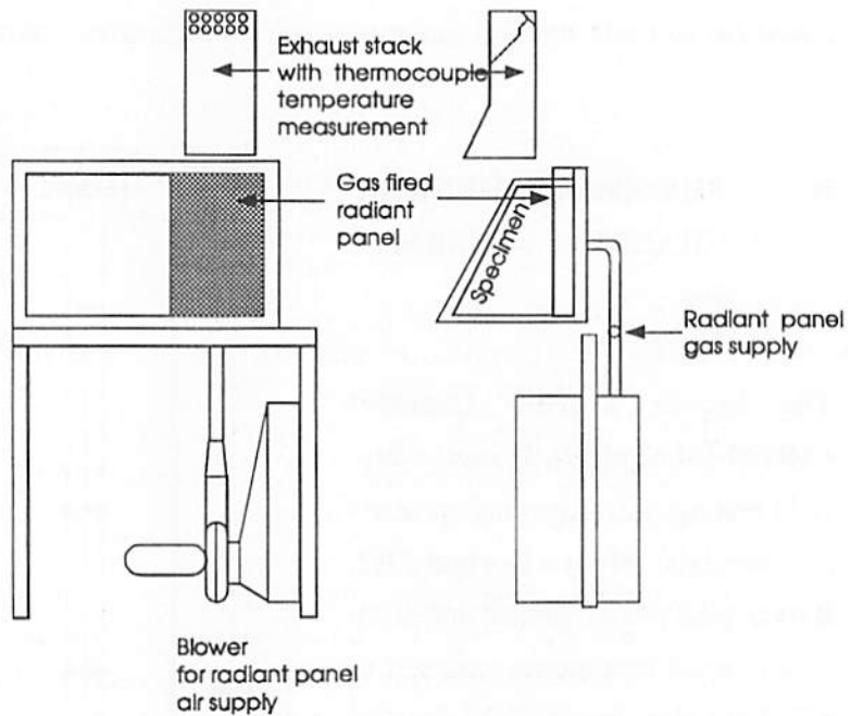
Figure B1. The ASTM E 162 Test for Surface Flammability of Materials Using a Radiant Heat Energy Source
