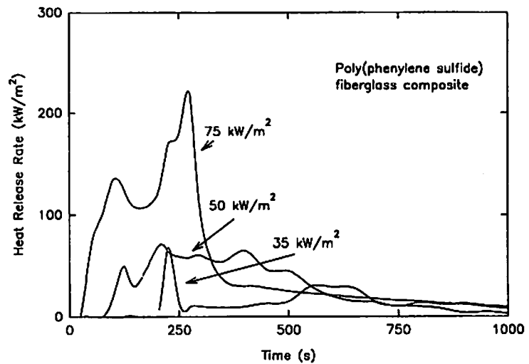
Figure 7. Example of the Effect of Irradiance on the Heat Release Rate for a Composite Material
