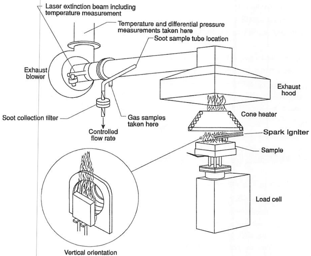
Figure 4. General View of the Cone Calorimeter (ASTM E 1354, ISO 5660).
