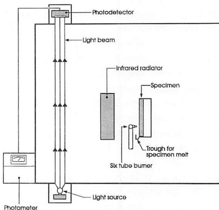
Figure B2. The ASTM E 662 Test for Specific Optical Density of Smoke Generated by Solid Materials
