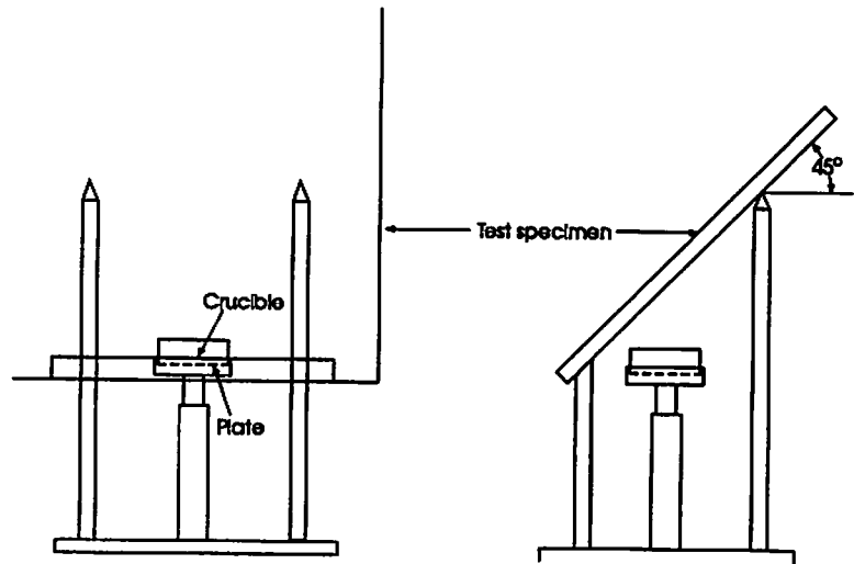
Figure D5. The UIC 564-2 Ignition Resistance Test
