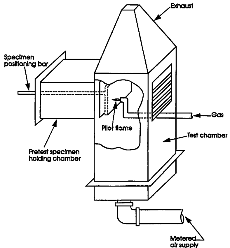
Figure D3. The OSU Calorimeter Test
