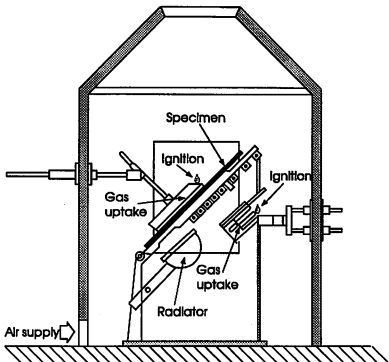
Figure C1. The NF P 92501 Epiradiateur Flammability Test
