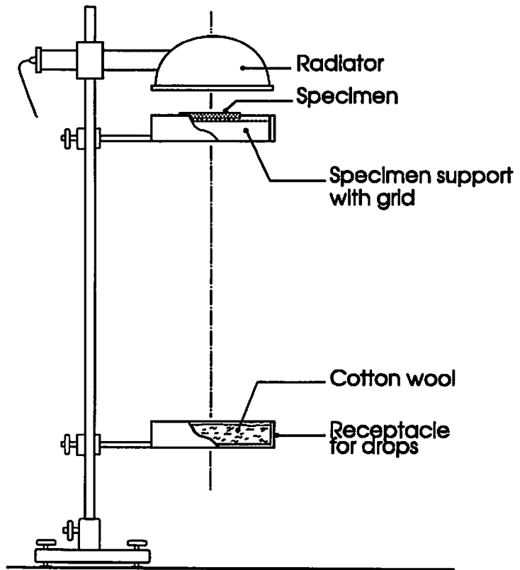
Figure C4. The NF P 92505 Dripping Test
