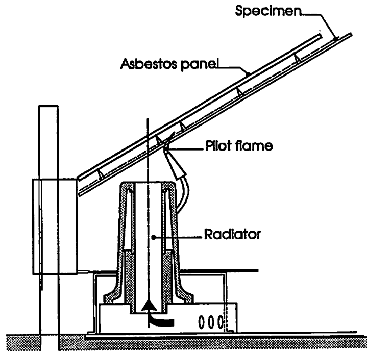
Figure C2. The NF P 92503 Burner Test for Flexible Materials
