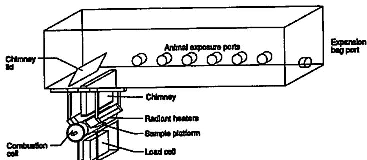
Figure 1. General View of the Radiant Toxicity Apparatus
