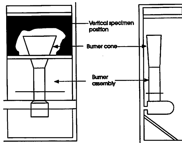
Figure D4. The FAR 25.853 Heat Conduction Test
