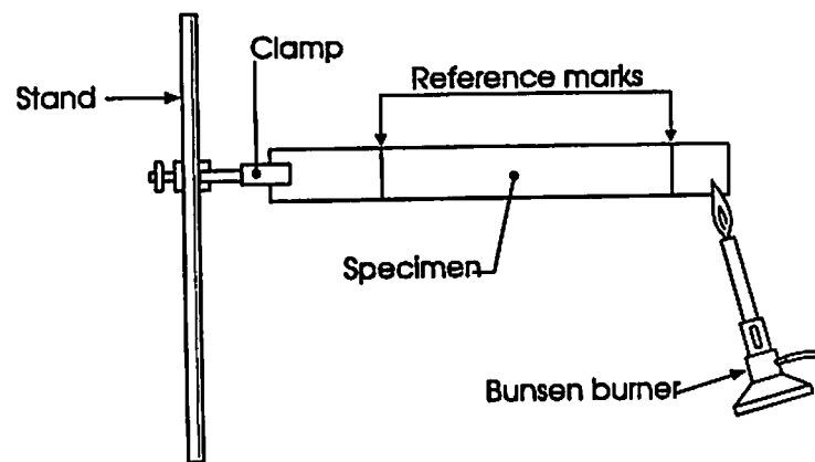
Figure C3. The NF P 92504 Bunsen Burner Test for Small-ignition Source Flammability
