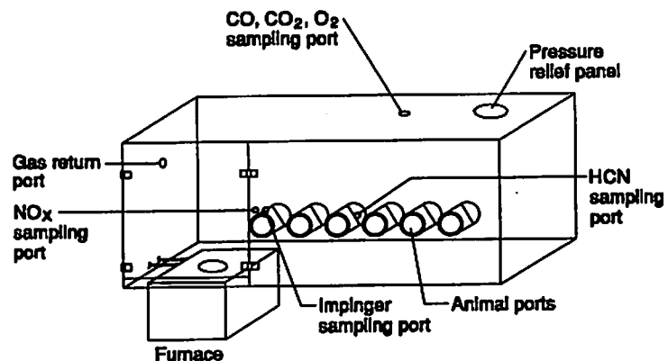
Figure B5. The Closed-System Cup Furnace Toxicity Method
