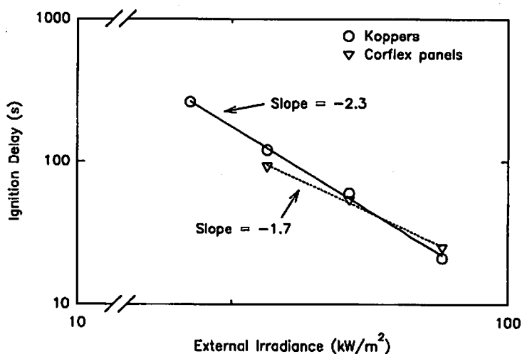
Figure 6. Time to Ignition as a Function of Irradiance for Two Different Composite Panels
