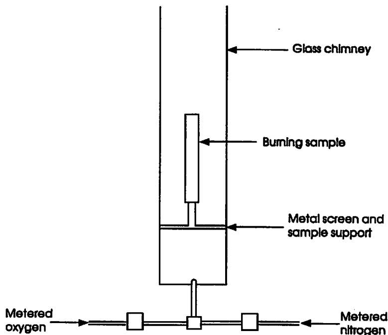
Figure C6. The NF T 51071 Oxygen Index Test for Small Samples
