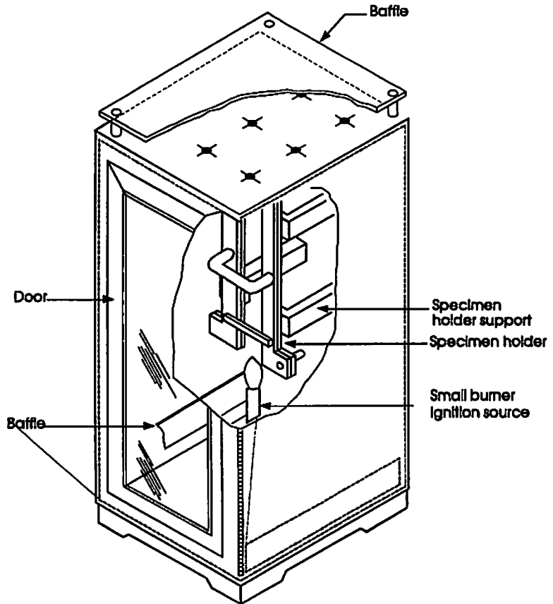
Figure B4. The FAR 25.853 Test, a Vertical Bunsen-Burner Test
