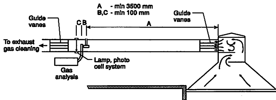
Exhaust Hood Calorimeter
