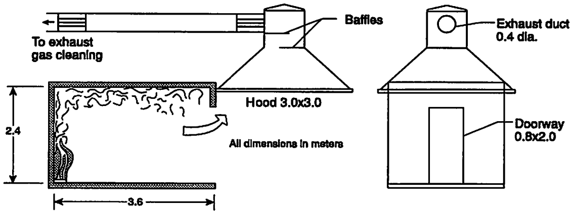
Test Room Configuration
