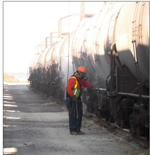
Figure 14: Inspect Rail Tank Car
